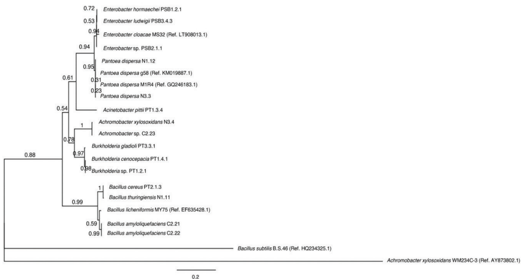
Figure 7: Phylogenetic tree of 15 bacterial strains and six reference strains
