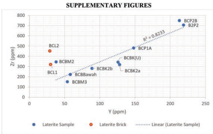
Figure S1: Two-dimensional scatter plot for concentration of immobile elements (Zr vs Y)
