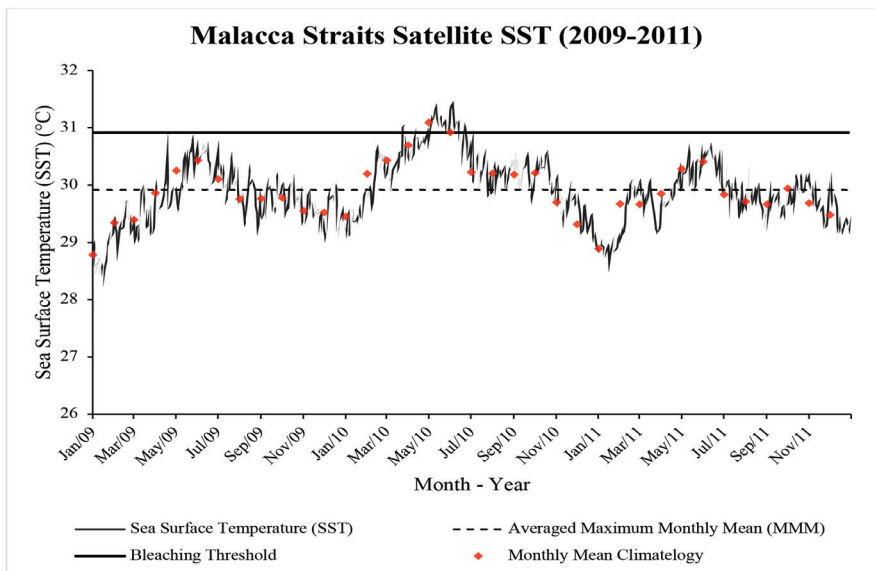
Figure 3 (a): Malacca Strait Satellite Sea Surface Temperatures (SST) (January 2009–December 2011)
