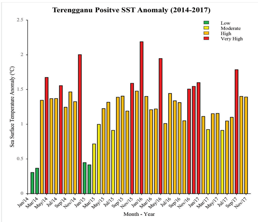
Figure 6 (b): Terengganu Satellite Sea Surface Temperatures (SST) anomaly based on their intensity (January 2014–December 2017) Source: NOAA Pathfinder CRW Program
