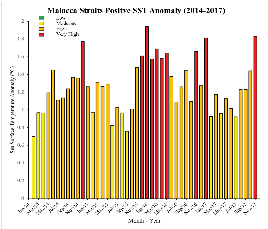
Figure 7 (b): Malacca Strait Satellite Sea Surface Temperatures (SST) anomaly based on their intensity (January 2014 – December 2017) Source: NOAA Pathfinder CRW Program
