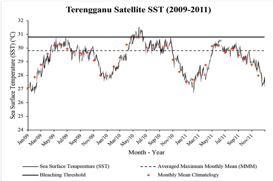
Figure 2 (a): Terengganu Satellite Sea Surface Temperatures (SST) (January 2009–December 2011) Source: NOAA Pathfinder CRW Program
