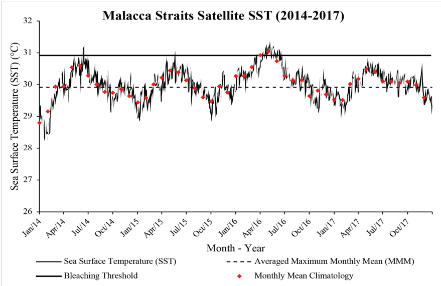
Figure 7 (a): Malacca Strait Satellite Sea Surface Temperatures (SST) (January 2014 – December 2017) Source: NOAA Pathfinder CRW Program
