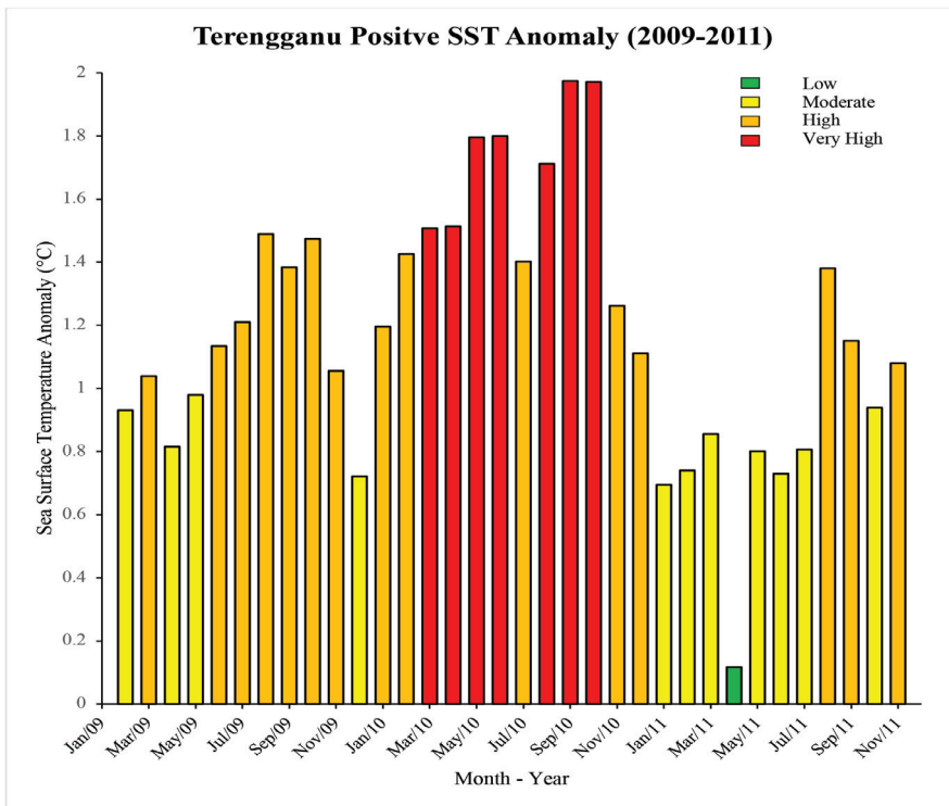
Figure 2 (b): Terengganu Satellite Sea Surface Temperatures (SST) anomaly based on their intensity (January 2009 – December 2011) Source: NOAA Pathfinder CRW Program
