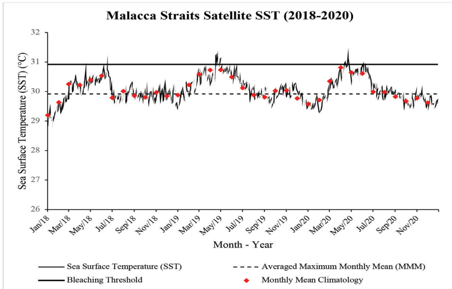
Figure 12 (a): Malacca Strait Satellite Sea Surface Temperatures (SST) (January 2018–December 2020) Source: NOAA Pathfinder CRW Program
