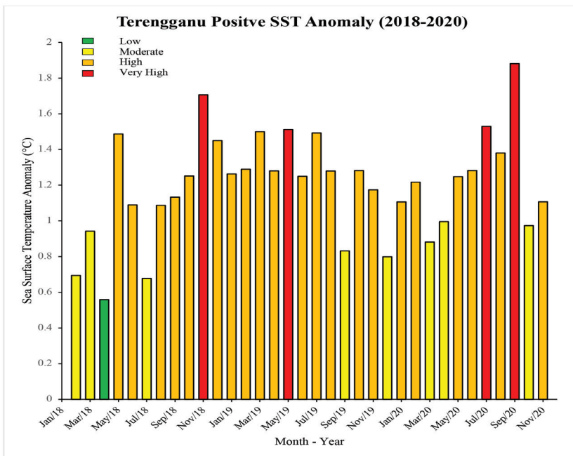
Figure 11 (b): Terengganu Satellite Sea Surface Temperatures (SST) anomaly based on their intensity (January 2018–December 2020) Source: NOAA Pathfinder CRW Program
