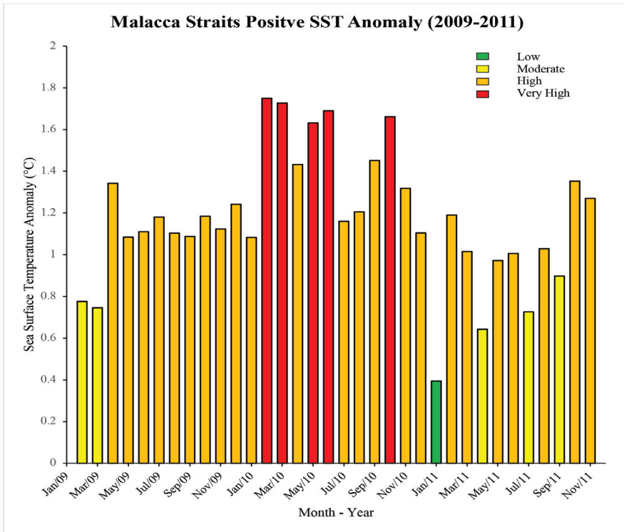
Figure 3 (b): Malacca Strait Satellite Sea Surface Temperatures (SST) anomaly based on their intensity (January 2009 – December 2011) Source: NOAA Pathfinder CRW Program
