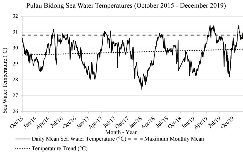
Figure 14: Pulau Bidong Sea Water Temperatures (October 2015 – December 2019). (Data Source: Pulau Bidong in-situ HOBO Logger, Universiti Malaysia Terengganu)
