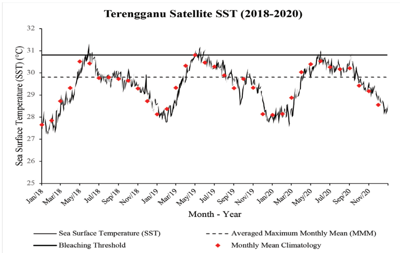
Figure 11 (a): Terengganu Satellite Sea Surface Temperatures (SST) (January 2018 – December 2020) Source: NOAA Pathfinder CRW Program
