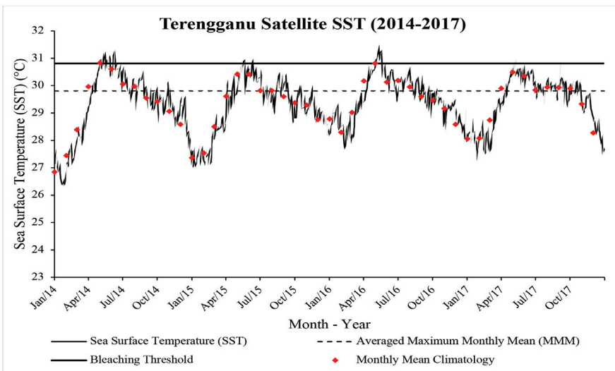
Figure 6 (a): Terengganu Satellite Sea Surface Temperatures (SST) (January 2014–December 2017) Source: NOAA Pathfinder CRW Program
