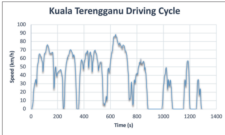
Figure 4: Proposed Kuala Terengganu driving cycle
