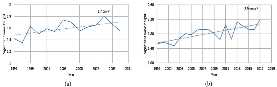
Figure 2: Annual variations in significant wave height. (a) Data set 1, (b) Data set 2
