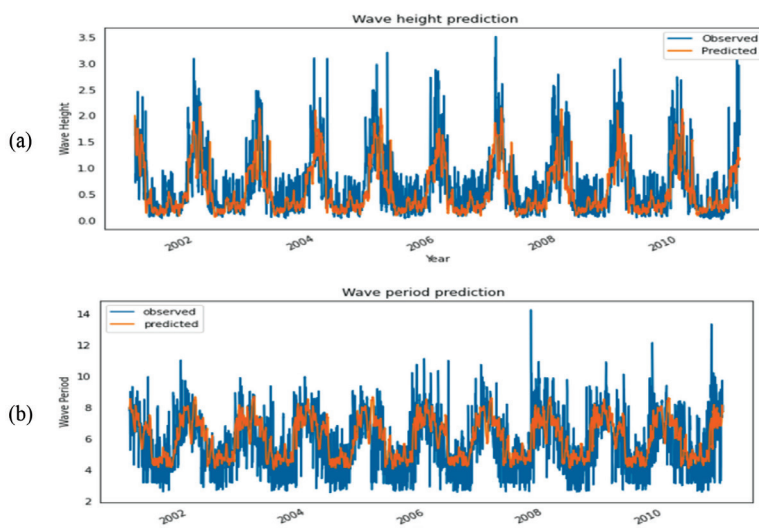
Figure 14: The add-and-repeat prediction results of data set 1. (a) The time series plots for observed and predicted wave height, and (b) the time series plots for observed and predicted wave period
