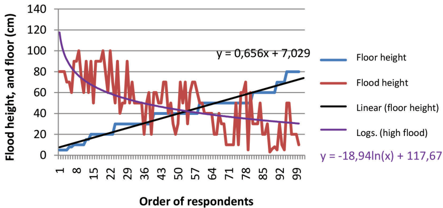
Figure 2: Drainage condition model against flood height
