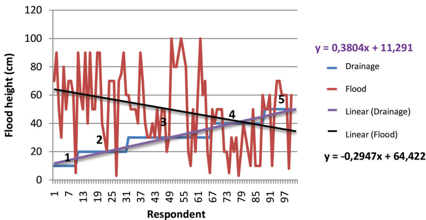
Figure 3: Mutual cooperation model against flood height
