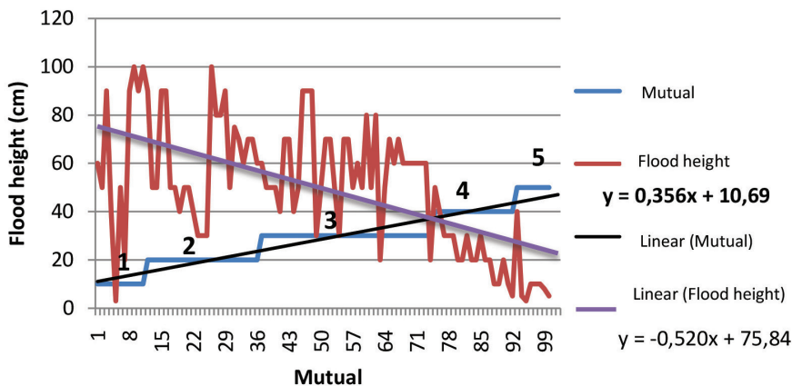
Figure 1: Model of house floor height against flood height
